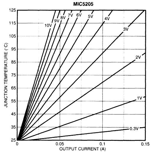
Figure 2-6 (C). SOT-23-5 with \theta_{JA} = 220^{\circ}C/W
