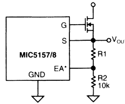
Figure 2. Typical Resistive Divider
