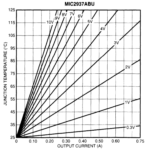
Figure 2-6 (G). TO-263 with \theta_{JA} = 40^{\circ}\text{C/W}
