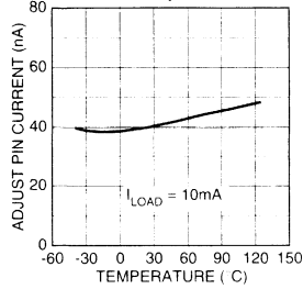
MIC29512 Adjust Pin Current vs. Temperature
