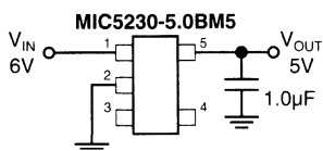
5V Linear Regulator Application
