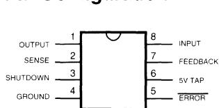
SO/DIP Packages (MIC29204BJ/M/N)
