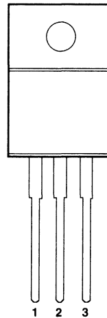
INPUT GROUND OUTPUT TO-220 Package (MIC2937A-xxBT)
