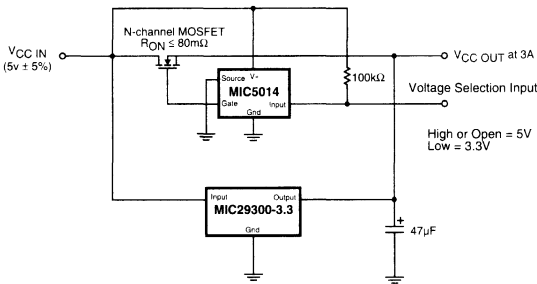
Figure 3-38. Switching 5V or 3.3V to a Microprocessor
