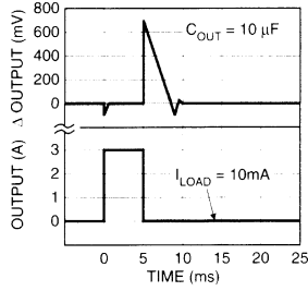
MIC2930x Load Transient
