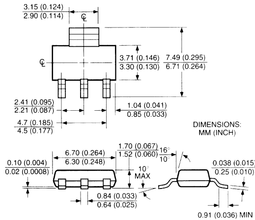
SOT-223 (S)
