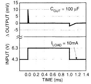
MIC2930x Line Transient
