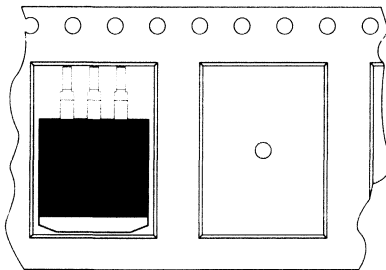
SOT-223 Package Orientation 16mm Carrier Tape
