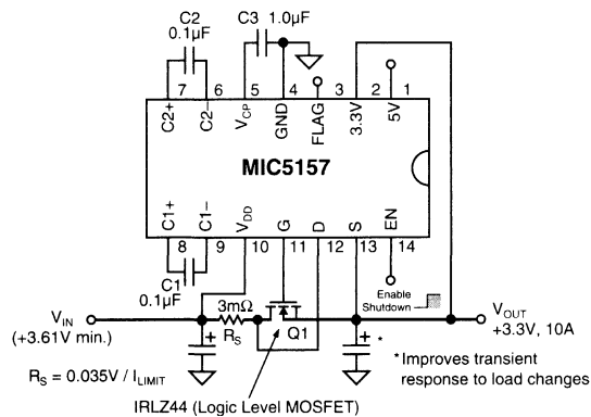
Figure 4-6. 10A Linear Regulator
