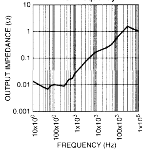
MIC2930x Output Impedance vs. Frequency
