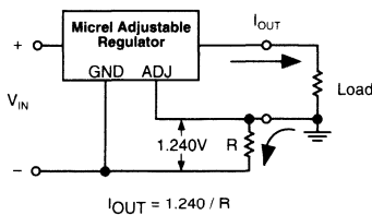
Figure 3-24. Simple Current Source Uses Reference Resistor in -V Return
