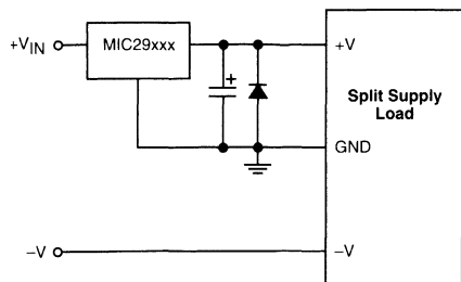
Figure 3-16. Diode Clamp Allows Start-Up in Split-Supply System
