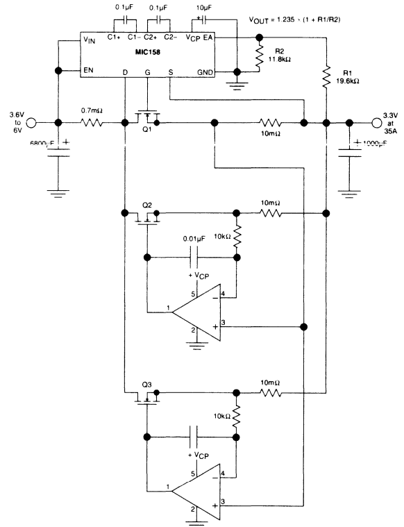
Figure 4-9. Parallel MOSFETs for High Current and/or High Power Dissipation Regulators
