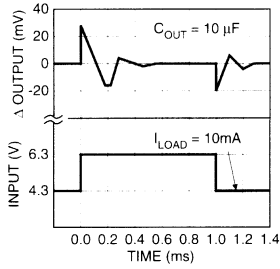
MIC2930x Line Transient
