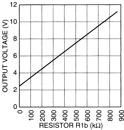
Figure 3-9. Output Voltage vs. R1b (See Figure 3-8)
