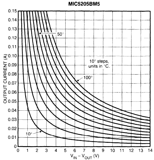
Figure 2-7 (C). SOT-23-5 with \theta_{JA} = 220^\circ\text{C/W}
