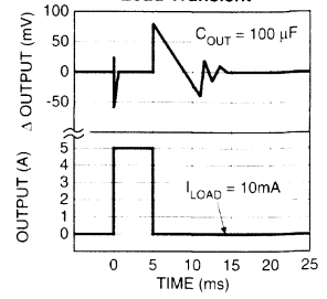
MIC2950x Load Transient
