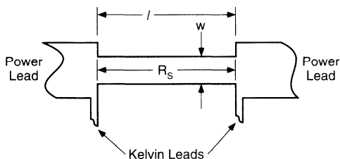
Figure 4-12. Typical Kelvin Resistor Layout
