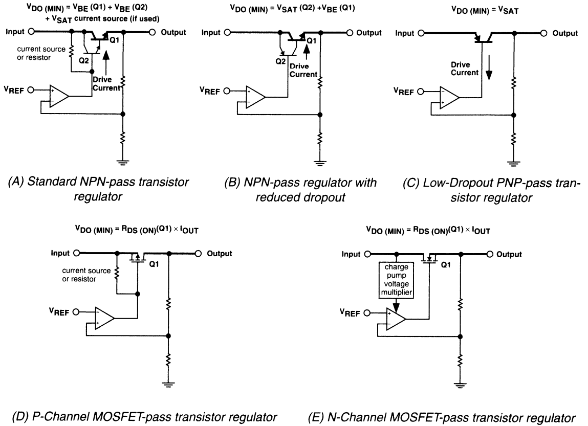
Figure 1-3. The Five Major Types of Linear Regulators
