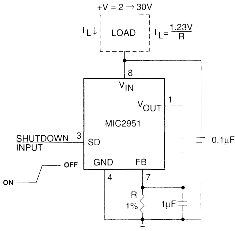
Low Drift Current Source
