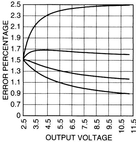
Figure 3-11. Composite Regulator Accuracy.
