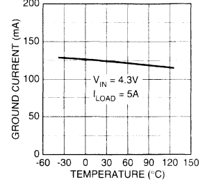
MIC2951x-3.3 Ground Current vs. Temperature
