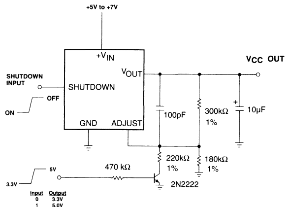
Figure 3. MIC29372/29373 Adjustable Regulator
