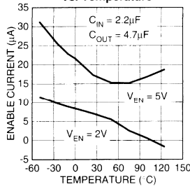
Enable Current Threshold vs. Temperature
