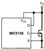
Figure 3. No Current Limit
