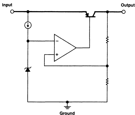
Figure 1-1. A basic linear regulator schematic.
