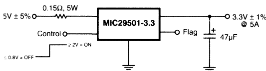
Figure 3-58. Resistor Power Sharing Reduces Heat Sink Requirement
