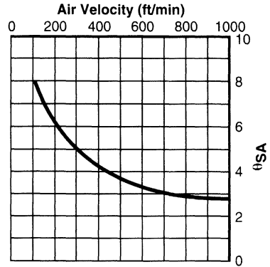
Figure 3-57. Forced Convection Performance
