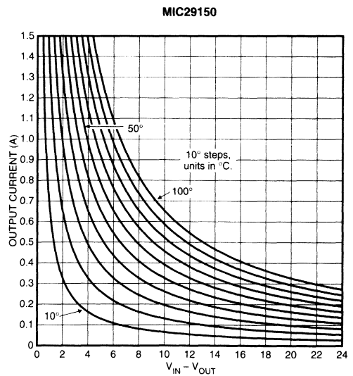
Figure 2-7 (H). TO-220 with \theta_{JA} = 15^{\circ}\text{C/W}
