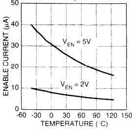
MIC29512 Enable Current vs. Temperature
