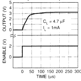
Enable Transient (3.3V Version)
