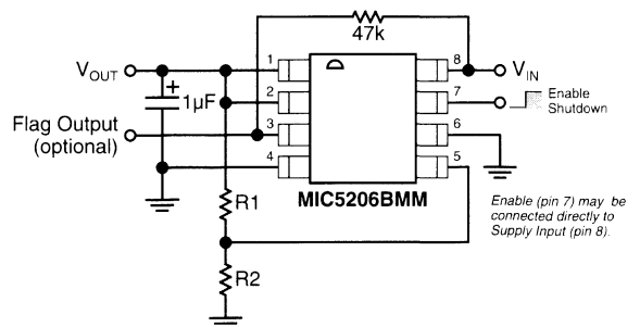
Micrel Mini8™ Adjustable Voltage Application
