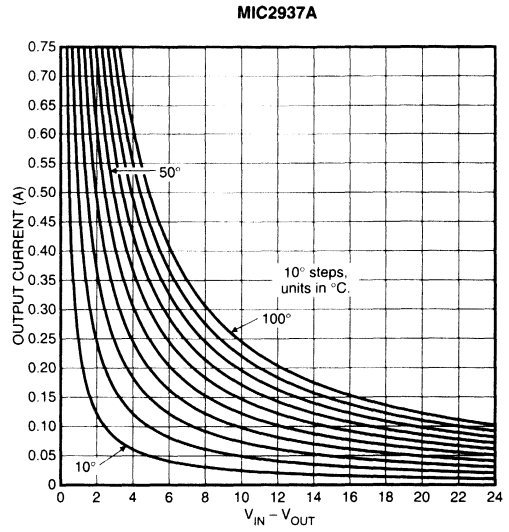
Figure 2-7 (G). TO-263 with \theta_{JA} = 40^{\circ}\text{C/W}
