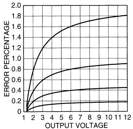
Figure 3-6. Resistor Tolerance Effects on Adjustable Regulator Accuracy
