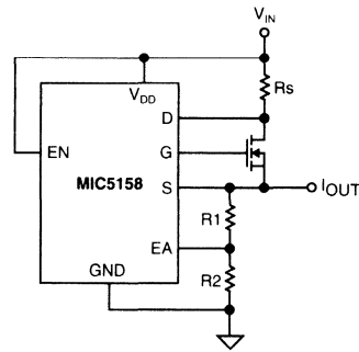
Figure 3-25. Simple Current Source Using the Super LDO
