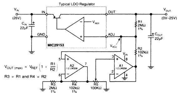
Figure 3-15. 0V-to-25V Adjustable Regulator
