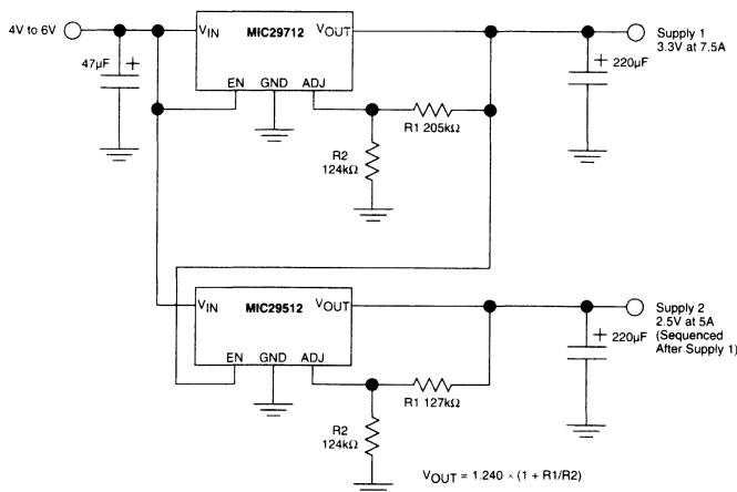
Figure 3-42. Multiple Supply Sequencing.
