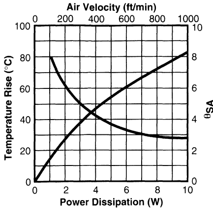
Figure 3-55. Typical Heat Sink Performance Graph
