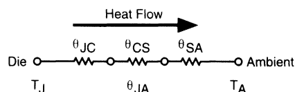
Figure 3-47. Heat flow through the interface resistances.
