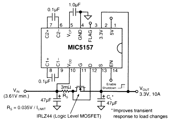
10A Low-Dropout Voltage Regulator
