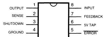
DIP and SO Packages (BN, and BM)
