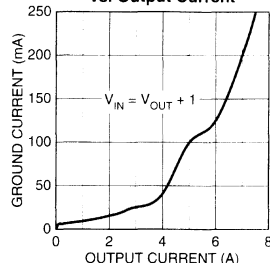
MIC29710/2 Ground Current vs. Output Current
