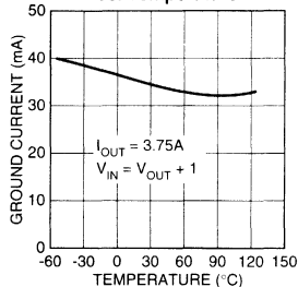
MIC29710/2 Ground Current vs. Temperature
