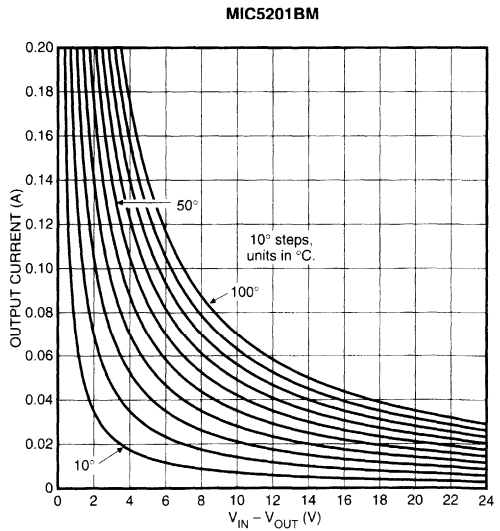
Figure 2-7 (D). SO-8 with \theta_{JA} = 140^\circ\text{C/W}
