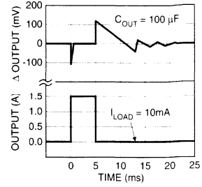
MIC2915x Load Transient
