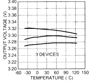
MIC29510-3.3 Output Voltage vs. Temperature
