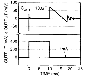
Load Transient
