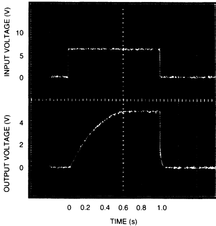
Figure 3-23. Turn-On Behavior of Figure 3-22.
