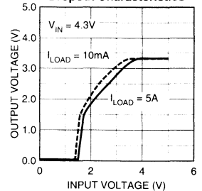
MIC29510-3.3 Dropout Characteristics
