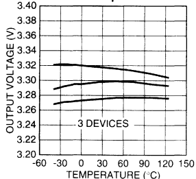
MIC29710-3.3 Output Voltage vs. Temperature
