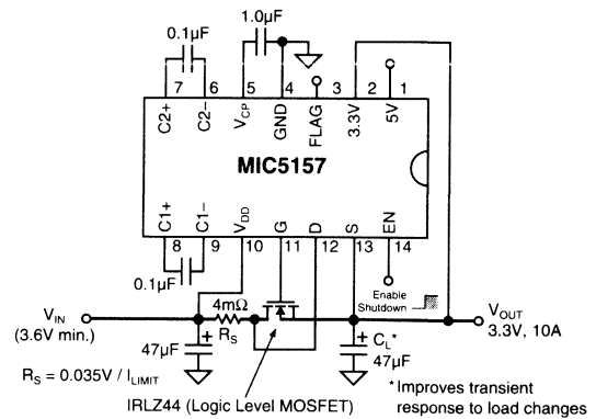
Figure 4-11. Regulator Circuit Diagram
