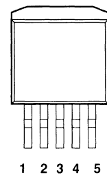
TO-263-5 Package (MIC29201/29202/29203BU)
