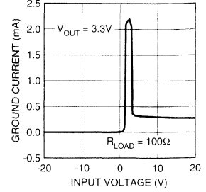
MIC2951x Ground Current vs. Input Voltage
