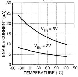
MIC29501-xx/2 Enable Current vs. Temperature
