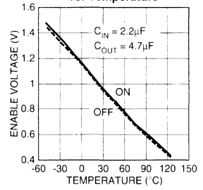
Enable Voltage Threshold vs. Temperature
