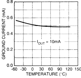
MIC2951x Ground Current vs. Temperature
