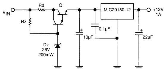
Figure 3-17. Preregulator Allows High Input Supply
