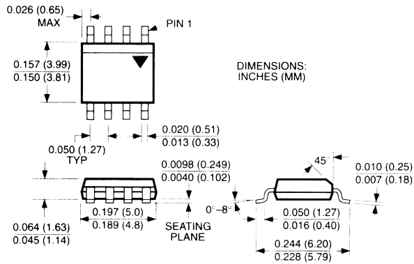
8-Pin SOIC (M)
