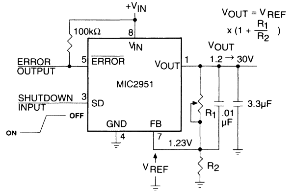
Figure 2. Adjustable Regulator
