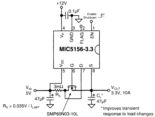
Figure 3-30. MIC5156 5V-to-3.3V Converter
