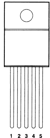
TO-220-5 Package (MIC29371/29372/29373BT)
