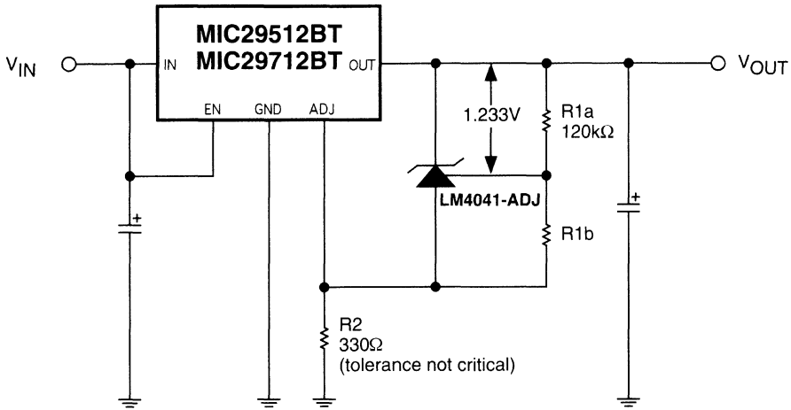
Figure 3-8. Improved Accuracy Composite Regulator Circuit
