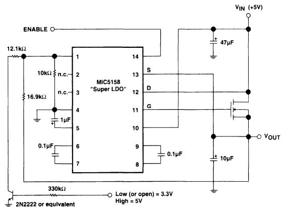
Figure 3-40. MIC5158 with Selectable Output Voltages
