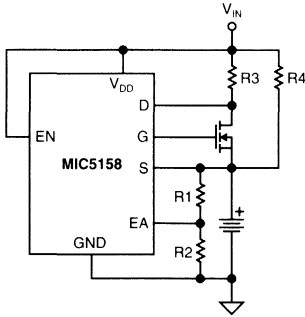
Figure 5. Battery Charger Concept
