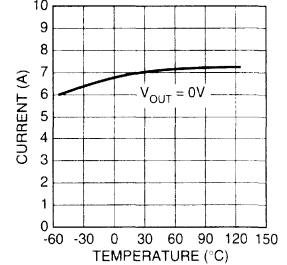
MIC2951x Short Circuit Current vs. Temperature
