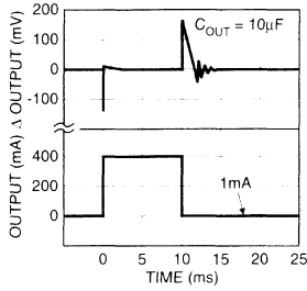
Load Transient
