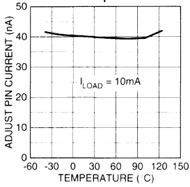
MIC29302/3 Adjust Pin Current vs. Temperature
