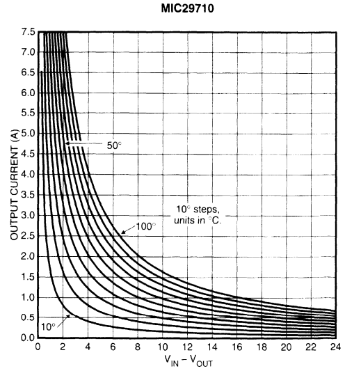
Figure 2-7 (K). TO-220 with \theta_{JA} = 6^{\circ}\text{C}/\text{W}
