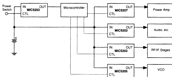
Figure 3-44. Cellular Telephone Block Diagram
