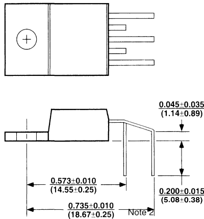
TO-220 Horizontal Lead Bend Option -LB02
