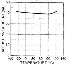
MIC29712 Adjust Pin Current vs. Temperature
