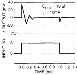
Line Transient
