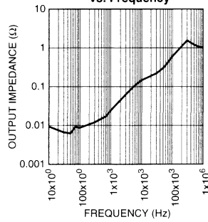
MIC2950x Output Impedance vs. Frequency
