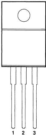
INPUT GROUND OUTPUT TO-220 Package (MIC2940A-xxBT)
