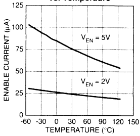
MIC29371/2 Shutdown Current vs. Temperature
