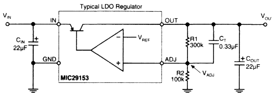
Figure 3-18. Simplest Slow Turn-On Circuit
