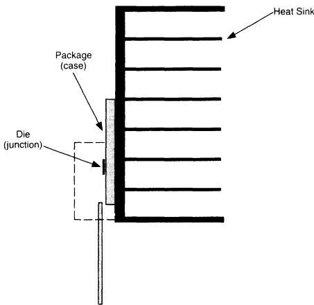
Figure 3-45. Regulator mounted to a heat sink.
