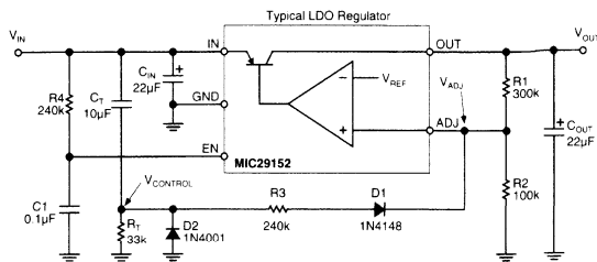
Figure 3-22. Slow Turn-On Without Pedestal Voltage
