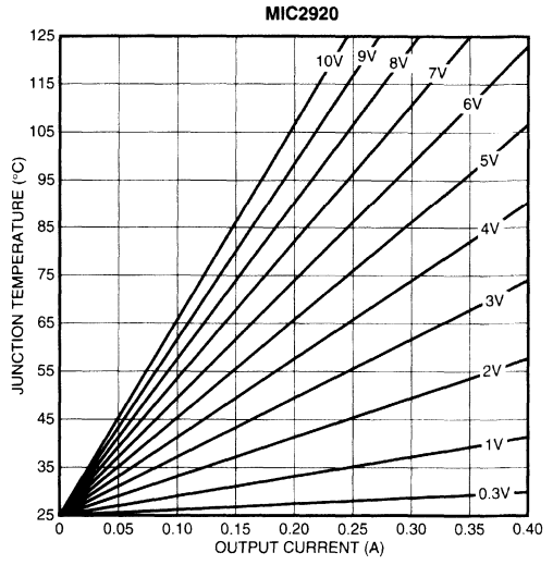
Figure 2-6 (F). TO-263 with \theta_{JA} = 40^{\circ}\text{C/W}
