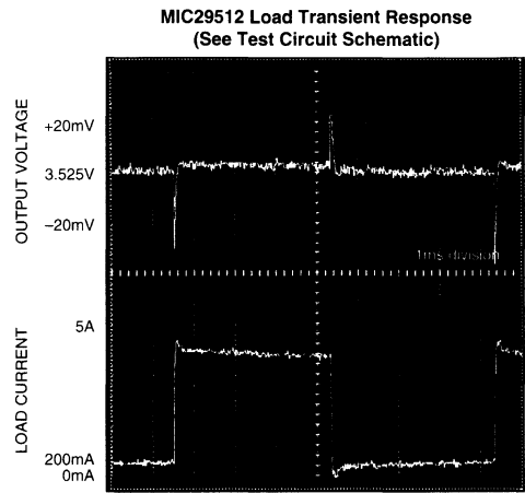
Figure 3-34. MIC29512 Load Transient Response.
