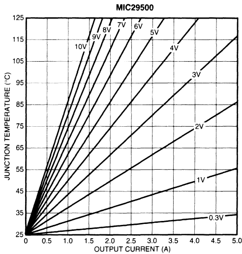
Figure 2-6 (J). TO-220 with \theta_{JA} = 6^{\circ}\text{C/W}
