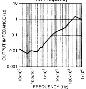
MIC29710/2 Output Impedance vs. Frequency
