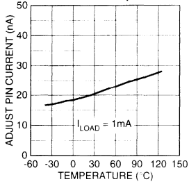
MIC29202/3 Adjust Pin Current vs. Temperature
