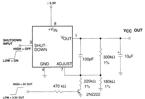
Figure 3. MIC29202/29203/29204 Adjustable Regulator. Pinout is for MIC29204.
