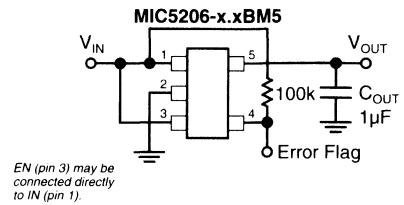
Figure 1a. Basic Fixed Voltage Application
