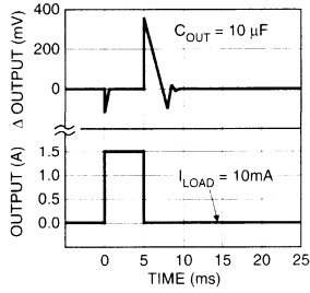
MIC2915x Load Transient
