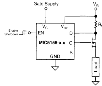
Figure 4a. High-Side Switch
