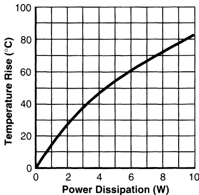
Figure 3-56. Natural Convection Performance
