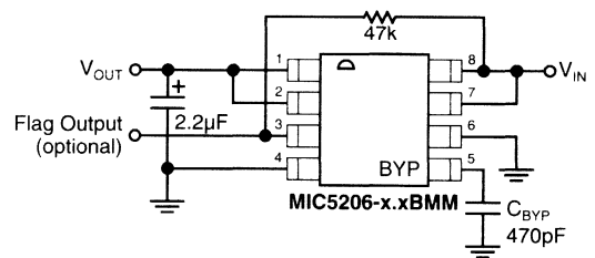
Figure 2. Low-Noise Fixed Voltage Application
