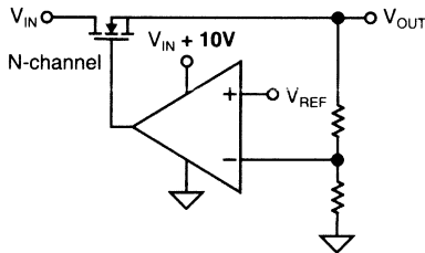
Figure 4-5. N-Channel Regulator
