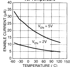
MIC29712 Enable Current vs. Temperature
