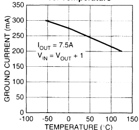
MIC29710/2 Ground Current vs. Temperature
