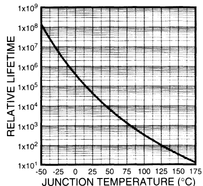
Figure 3-48. Typical MTTF vs. Temperature Curve.
