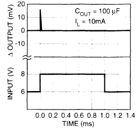
Line Transient
