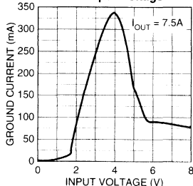
MIC29710/2 Ground Current vs. Input Voltage
