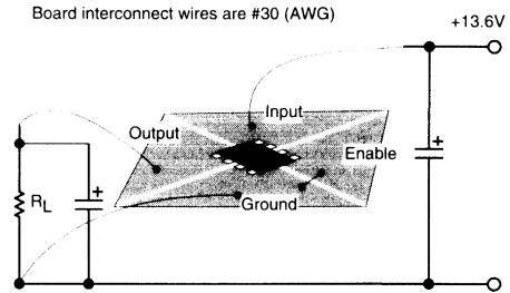
Figure 3-64. MSOP-8 Thermal Resistance Test Jig
