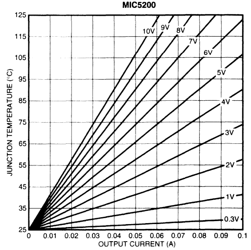
Figure 2-6 (B). SO-8 with \theta_{JA} = 160^{\circ}C/W
