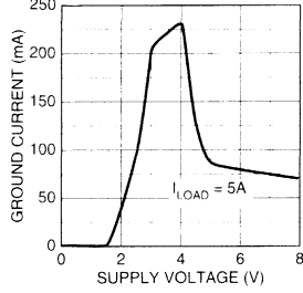
MIC2951x-3.3 Ground Current vs. Supply Voltage
