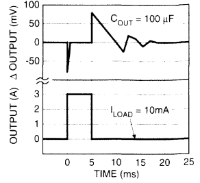
MIC2930x Load Transient
