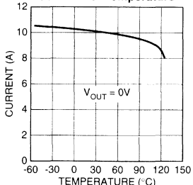
MIC29710/2 Short Circuit Current vs. Temperature
