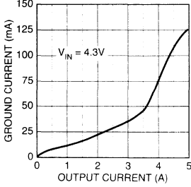
MIC2951x-3.3 Ground Current vs. Output Current
