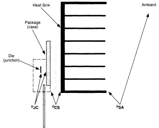
Figure 3-46. Thermal Parameters.
