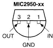
TO-92 (Z) (Bottom View)
