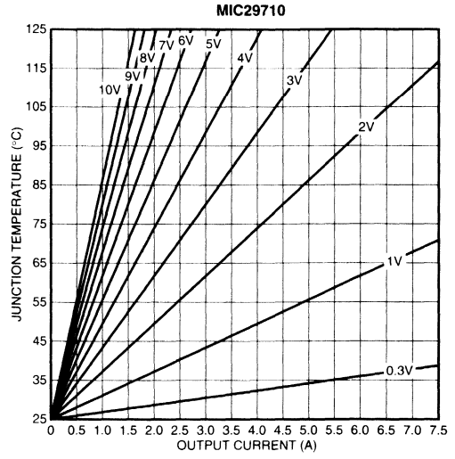
Figure 2-6 (K). TO-220 with \theta_{JA} = 6^{\circ}\text{C/W}
