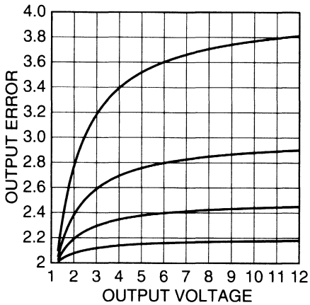
Figure 3-7. Worst-Case Output Tolerance.
