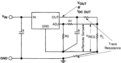
Figure 3-1. Remote Voltage Sense (Kelvin) Connections
