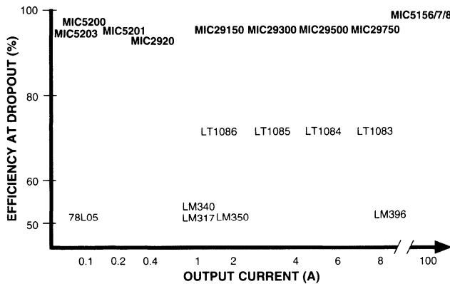
Figure 1-4. Linear Regulator Efficiency at Dropout
