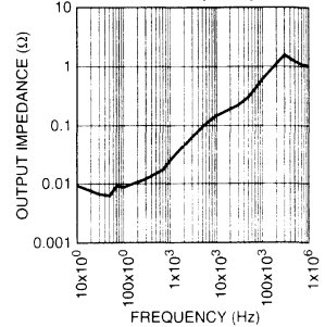
MIC2951x Output Impedance vs. Frequency
