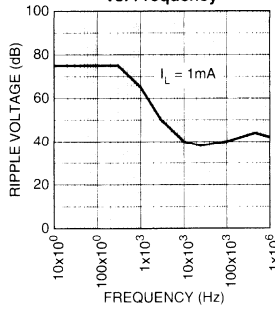
Ripple vs. Frequency
