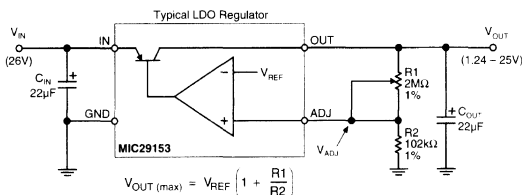
Figure 3-13. Typical Adjustable Regulator
