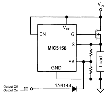
Figure 4b. Fast High-Side Switch
