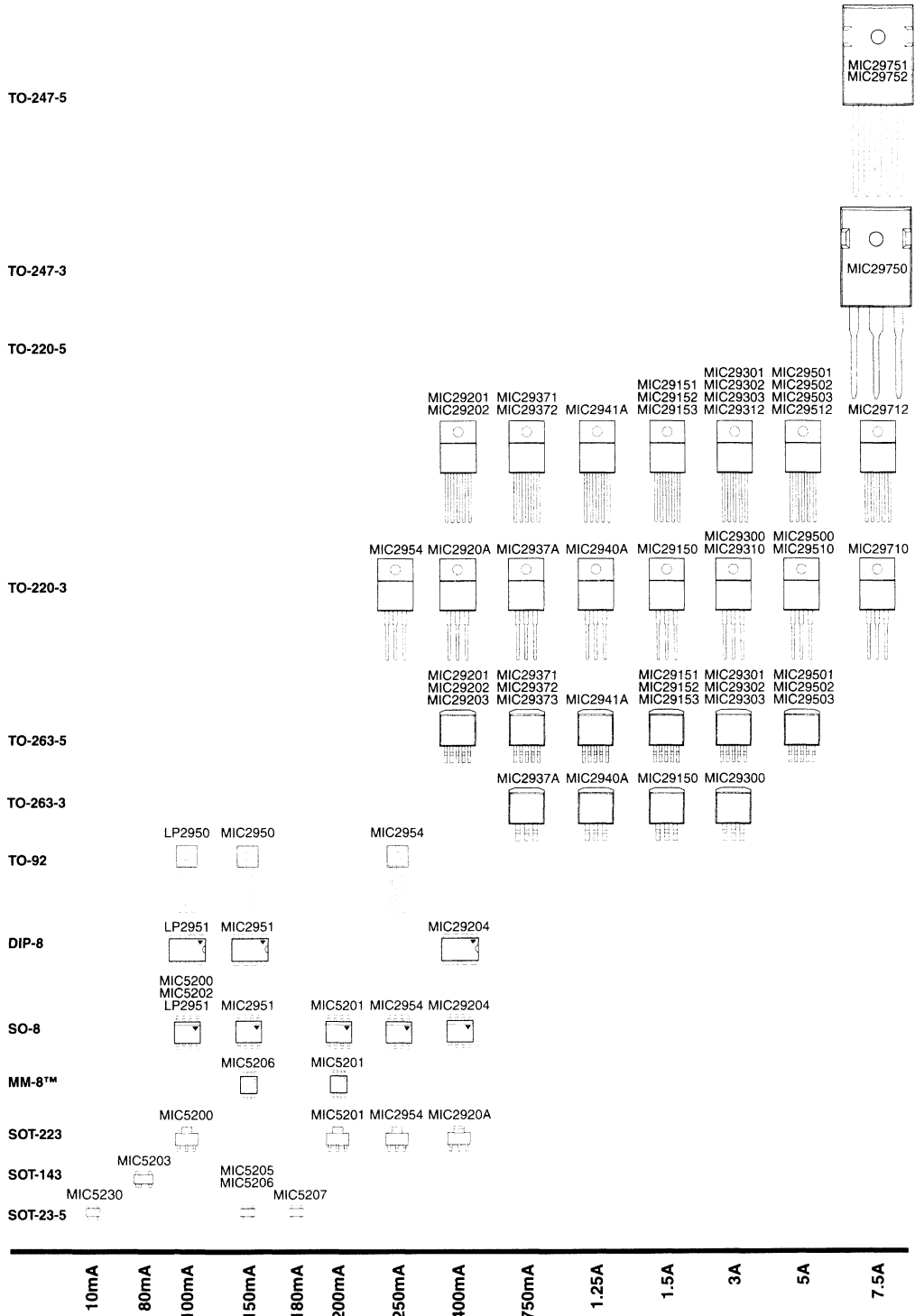
Figure 2-2. Output Current & Package Type Selector Guide
