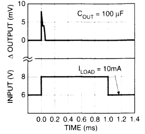
MIC2915x Line Transient
