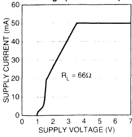
Supply Current vs. Supply Voltage (3.3V Version)
