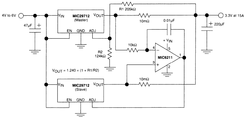
Figure 4-3. Two Super Beta PNP Regulators in Parallel.
