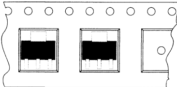
SOT-223 Package Orientation 16mm Carrier Tape
