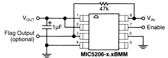
Figure 1b. Basic Fixed Voltage Application
