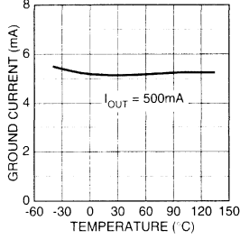
MIC2951x Ground Current vs. Temperature
