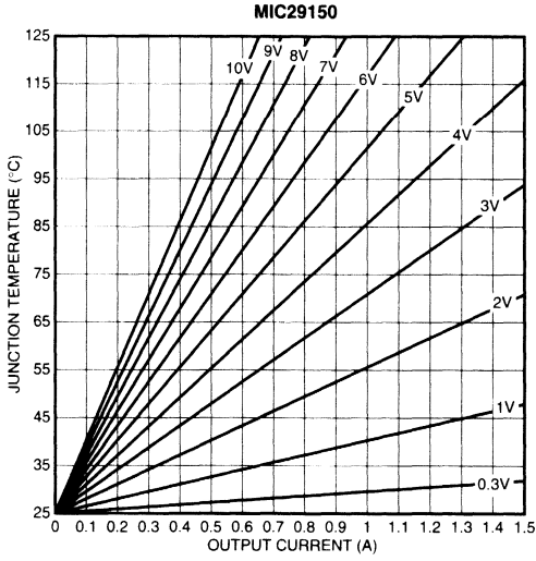
Figure 2-6 (H). TO-220 with \theta_{JA} = 15^{\circ}\text{C/W}
