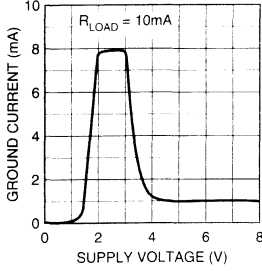
MIC2951x-3.3 Ground Current vs. Supply Voltage
