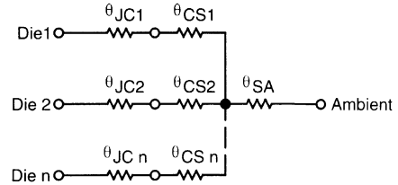
Figure 3-62. "n" Heat Source Thermal Circuit
