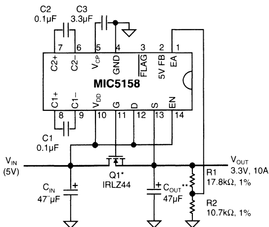
Figure 4-13. Simple 10A, 5V-to-3.3V Voltage Regulator
