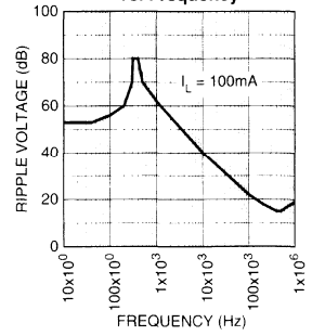
Ripple vs. Frequency
