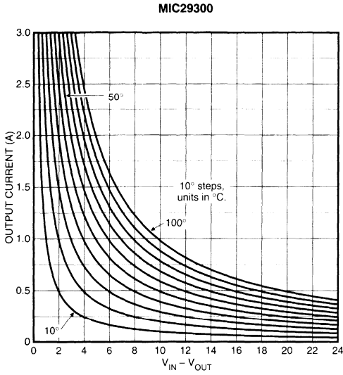
Figure 2-7 (I). TO-220 with \theta_{JA} = 10^{\circ}\text{C}/\text{W}
