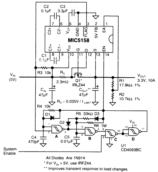
Figure 4-14. Short-Circuit Protected 10A Regulator
