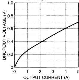
MIC2951x Dropout Voltage vs. Output Current
