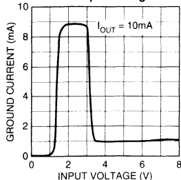
MIC29710/2 Ground Current vs. Input Voltage
