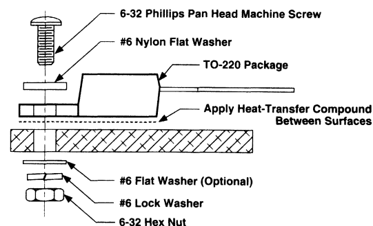
Figure 3-4. Mounting TO-220 Packages to Heat Sinks
