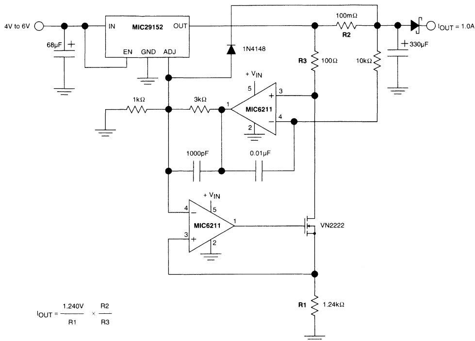
Figure 3-26. Current Source Using a Pair of Op-Amps
