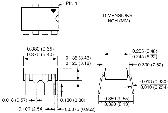
8-Pin Plastic DIP (N)
