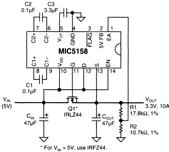
Figure 4-7. A High Current Regulator Using the MIC5158
