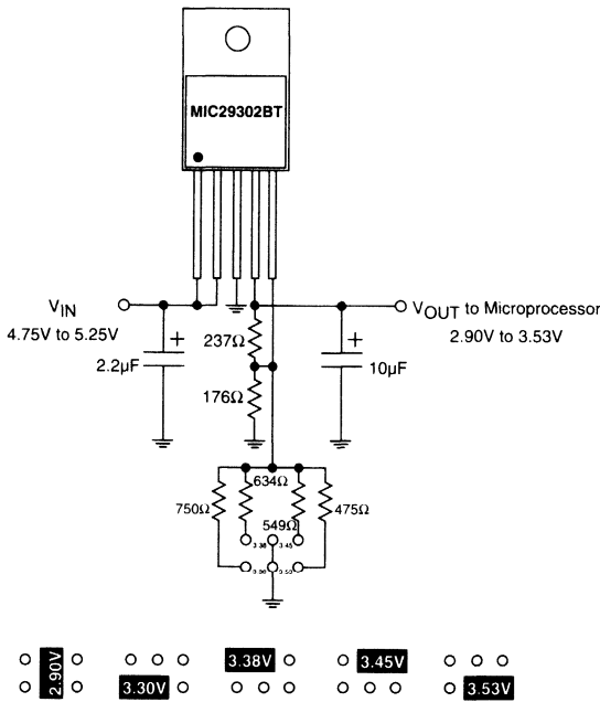
Voltage Jumper Positions
