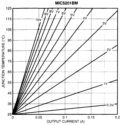
Figure 2-6 (D). High Current SO-8 with \theta_{JA} = 160^{\circ}\text{C/W}
