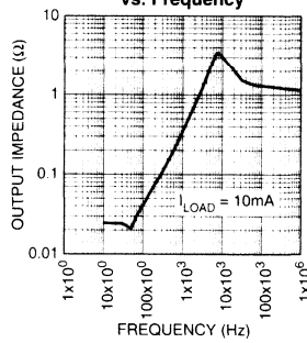
Output Impedance vs. Frequency
