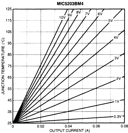
Figure 2-6 (A). SOT-143 with \theta_{JA} = 250^{\circ}C/W
