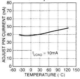
MIC29502/3 Adjust Pin Current vs. Temperature
