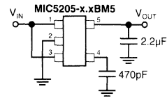
Figure 1. Low-Noise Fixed Voltage Application
