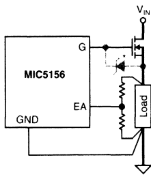
Figure 1b. Connections for Adjustable Output
