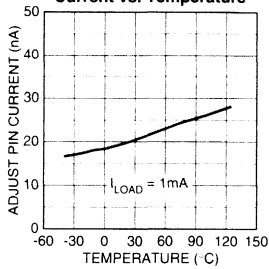
MIC29372/3 Adjust Pin Current vs. Temperature
