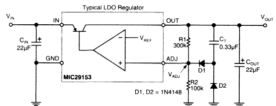
Figure 3-20. Improved Slow Turn-On Circuit
