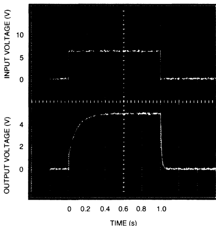
Figure 3-19. Turn-On Behavior for Circuit of Figure 3-18
