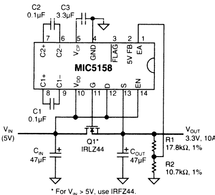
Figure 3-31. MIC5158 5V-to-3.3V Converter
