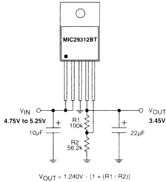
Figure 4. Adjustable Regulator with Resistors
