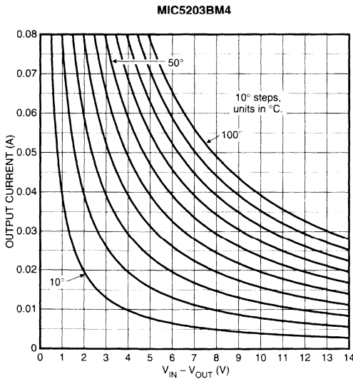
Figure 2-7 (A). SOT-143 with \theta_{JA} = 250^\circ\text{C/W}
