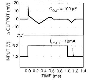
MIC2950x Line Transient
