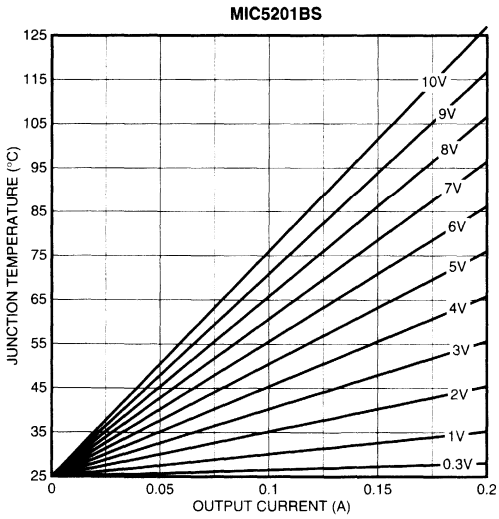
Figure 2-6 (E). SOT-223 with \theta_{JA} = 50^{\circ}\text{C/W}
