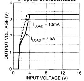
MIC29710-3.3 Dropout Characteristics
