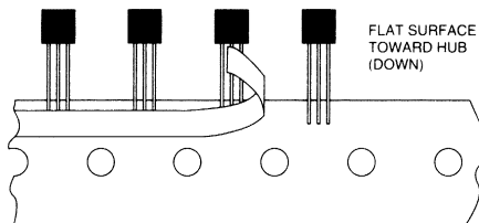
Typical TO-92 Package Orientation
