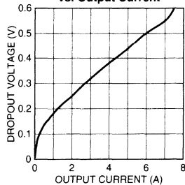
MIC29710/2 Dropout Voltage vs. Output Current
