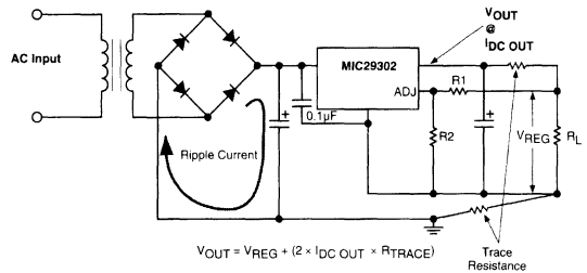
Figure 3-3. Regulator Layout With Remote Voltage Sensing
