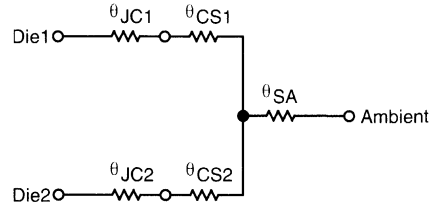
Figure 3-61. Dual Heat Source Thermal "Circuit"
