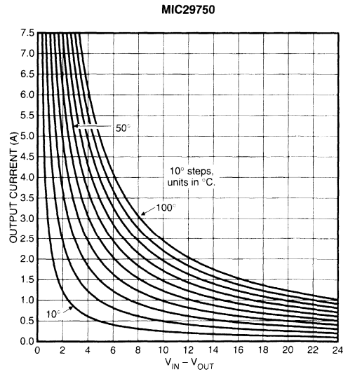
Figure 2-7 (L). TO-247 with \theta_{JA} = 4^{\circ}\text{C}/\text{W}
