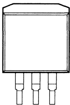
INPUT GROUND OUTPUT TO-263 Package (MIC2937A-xxBU)
