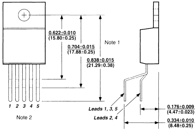
TO-220 Vertical Lead Bend Option -LB03
