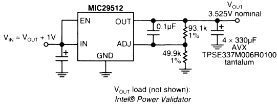
MIC29512 Load Transient Response Test Circuit
