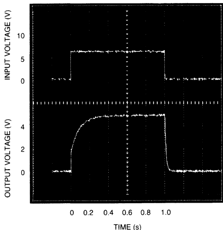
Figure 3-21. Turn-On Behavior of Figure 3-20.
