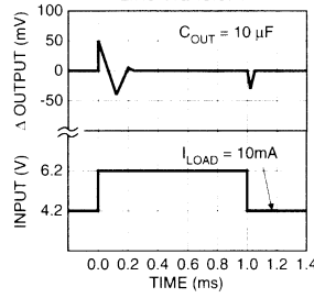
MIC2950x Line Transient
