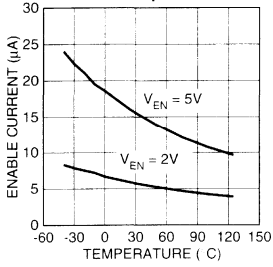
MIC29301-x/2 Enable Current vs. Temperature
