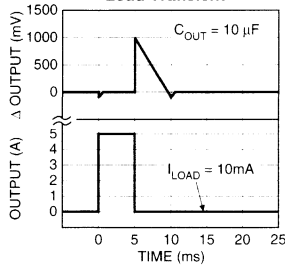
MIC2950x Load Transient
