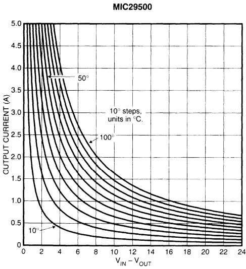
Figure 2-7 (J). TO-220 with \theta_{JA} = 6^{\circ}\text{C}/\text{W}
