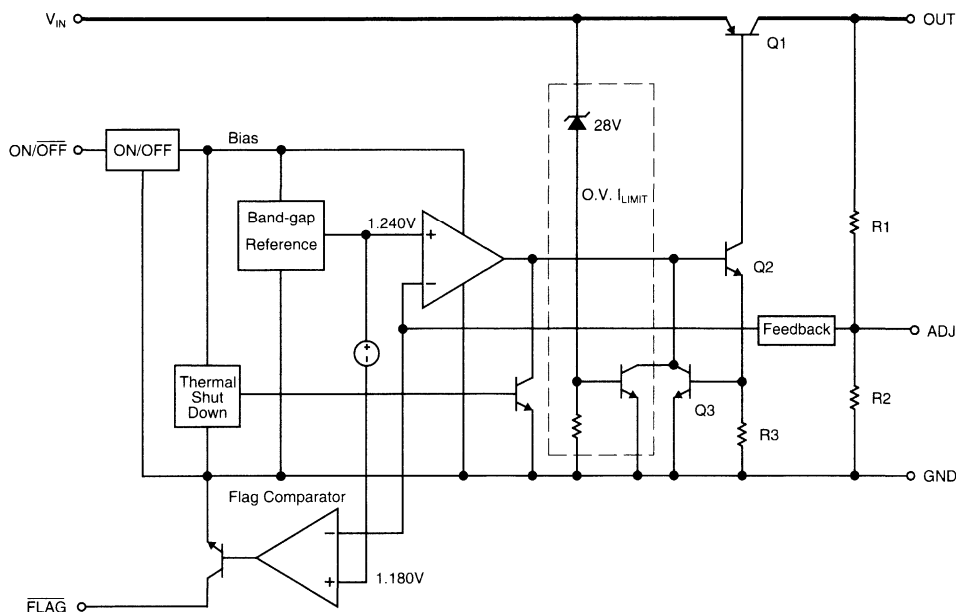
Figure 4-1. Super Beta PNP™ Regulator Simplified Schematic Diagram
