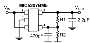
Figure 3. Low-Noise Adjustable Voltage Application
