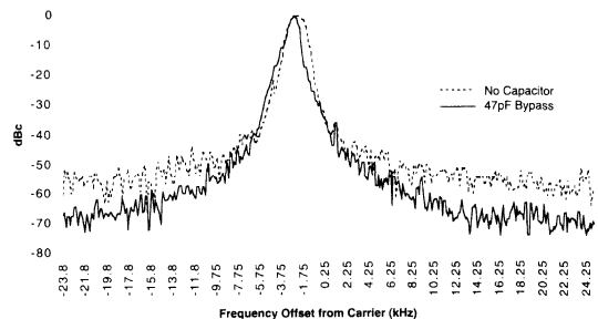
Figure 3-43. A Low Noise LDO (MIC5205) Reduces VCO Phase Noise.
