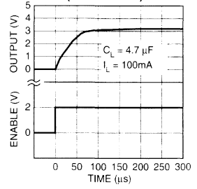
Enable Transient (3.3V Version)
