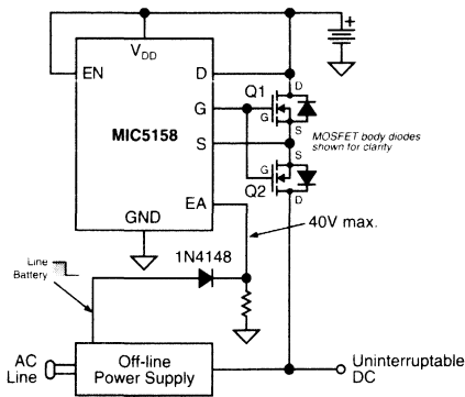
Figure 6. UPS Power Supply Concept
