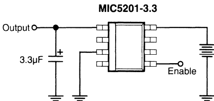
MIC5201 Fixed voltage application.
